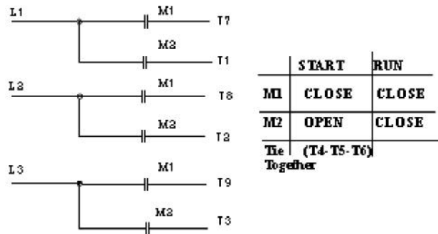
C-2 Part Winding Start (Low Voltage only)
